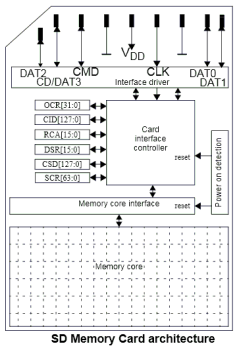
SD Memory Card architecture
